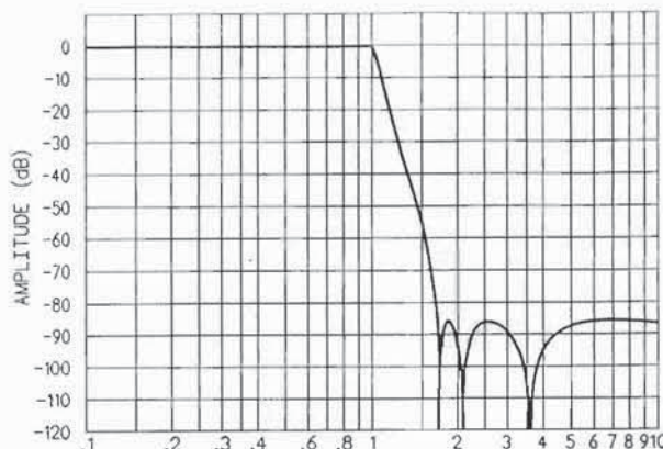
Figure 2.1 Amplitude Response
