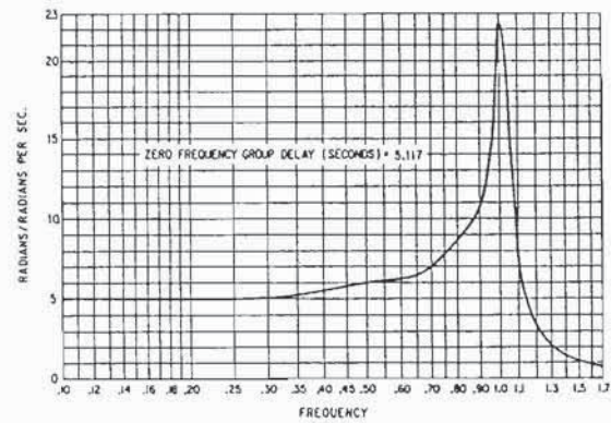
Figure 2.3 Group Delay
